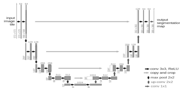
Figure 1. U-Net architecture Source: Zvarg, J. 2019
